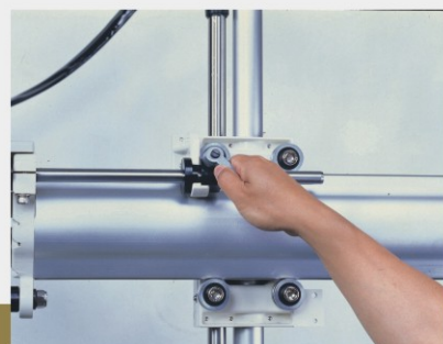
Tool-free adjustment on kick stroke.
